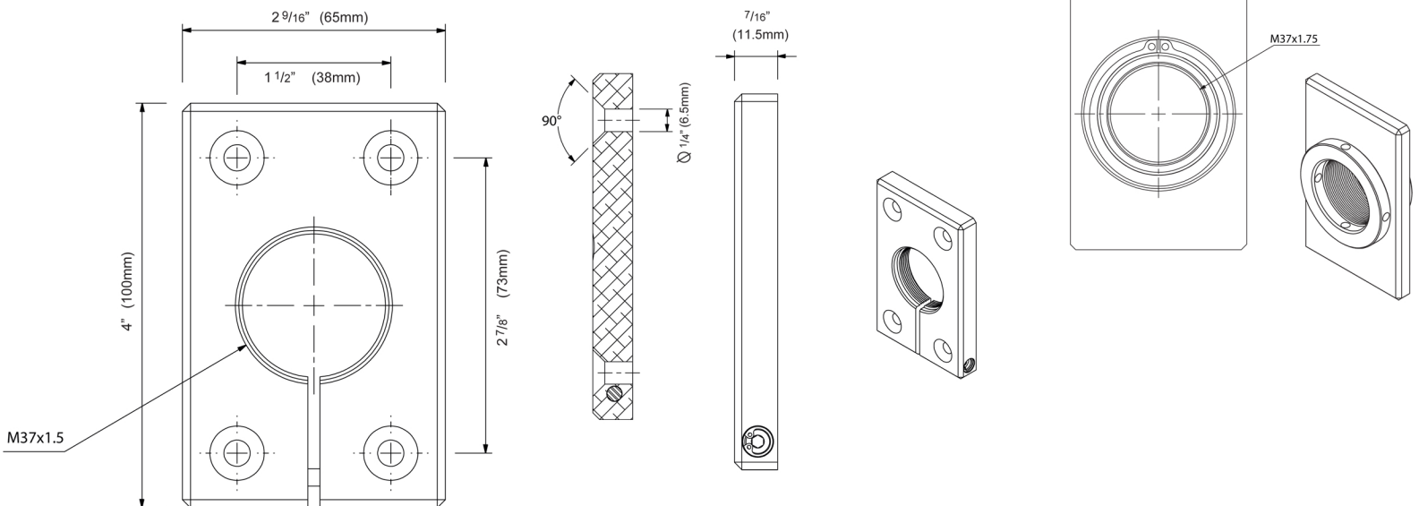
7514 - Bracket Type: 6026-04 Center Mount
