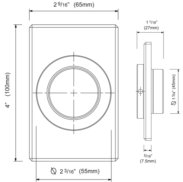
7526 - Bracket Type: 0510-05 Center Mount
