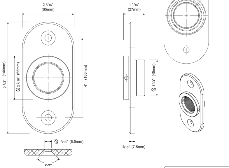
7513 - Bracket Type: 6026-03 Center Mount
