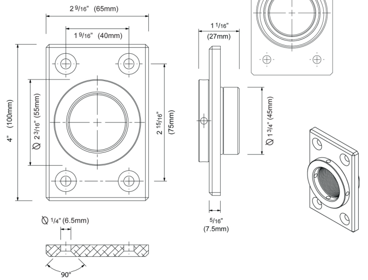
7526 - Bracket Type: 0510-05 Center Mount
