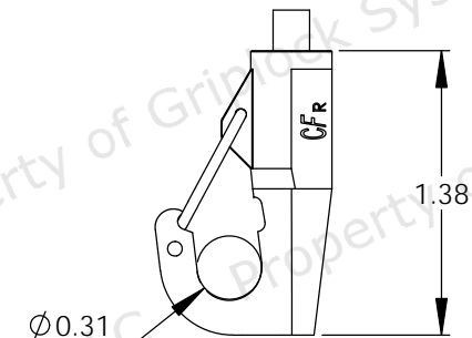
Gate Closed
